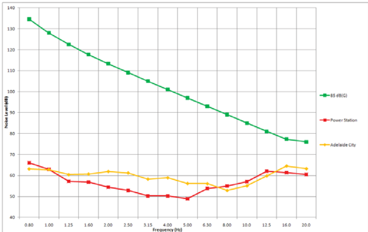
Figure 5. Measured levels of infrasound from engineered sources
